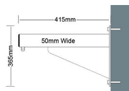
Bulkhead offset brackets
